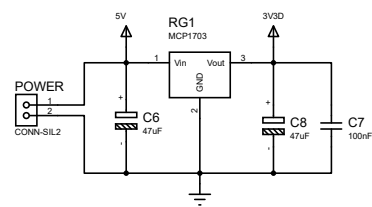
5V Power In
