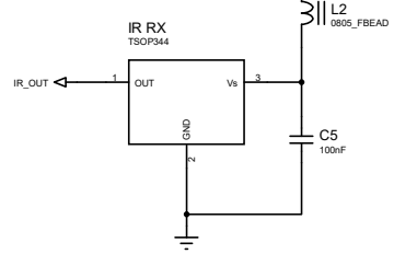
IR Receiver
