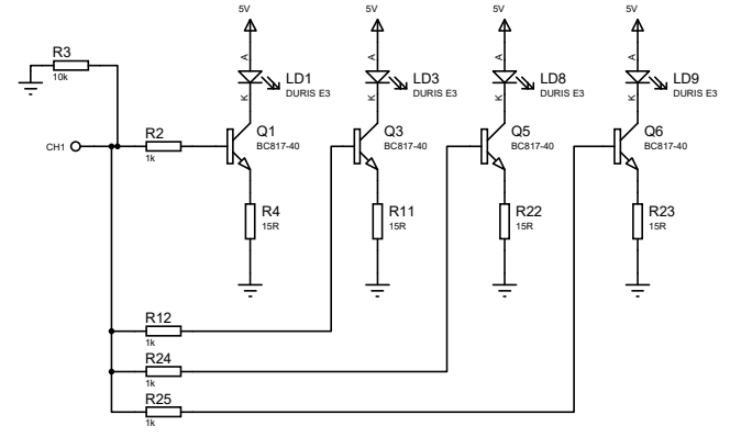
Red LEDs
