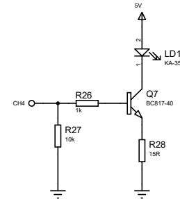
Green LEDs
